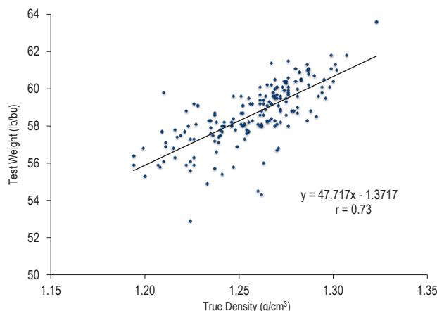
Test Weight vs True Density U.S. Aggregate 2025
